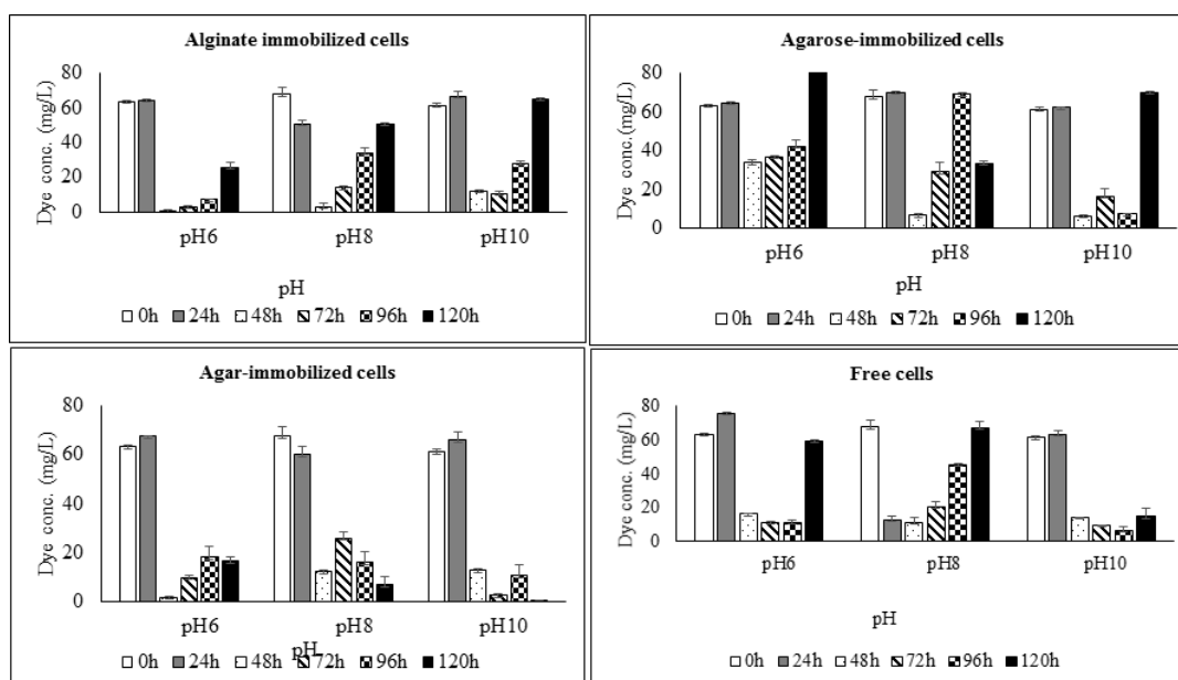
Fig. 1. Effect of pH on crystal violet concentration in the media in presence of the immobilized and free cells of the Pseudomonas aeruginosa
