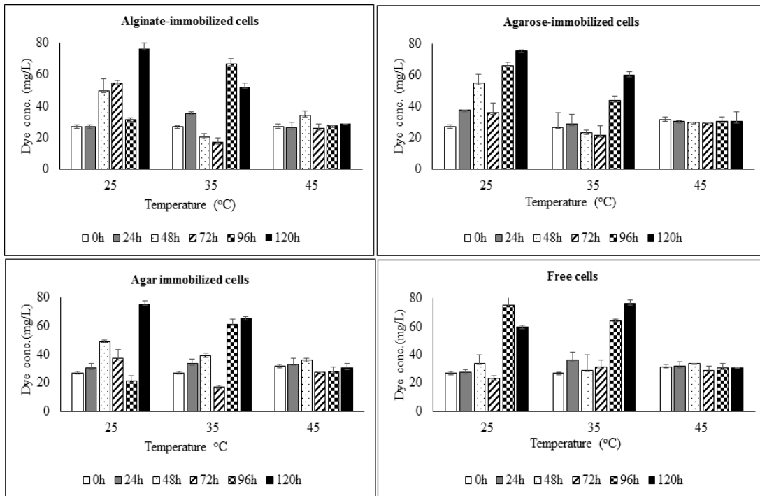
Fig. 2. Effect of temperature on crystal violet concentration in the media in presence of the immobilized and free cells of the Pseudomonas aeruginosa
