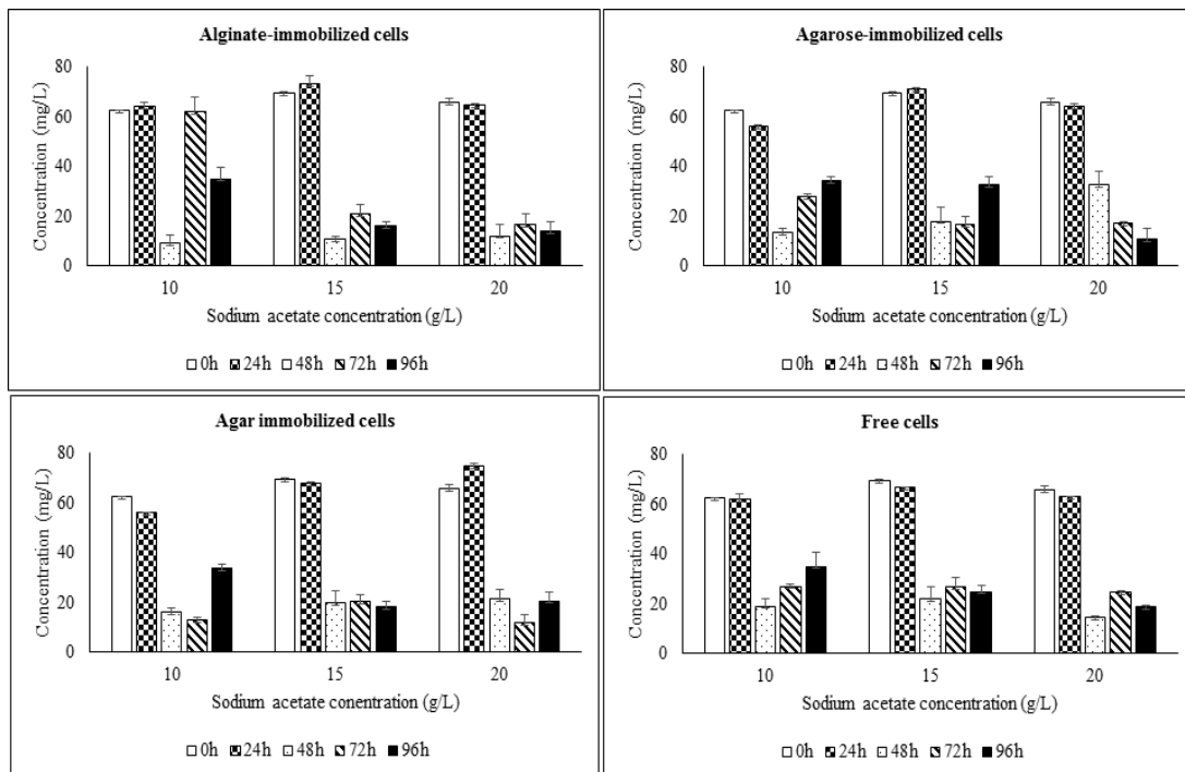
Fig. 3. Effect of sodium acetate concentration on crystal violet concentration in the media in presence of the immobilized and free cells of the Pseudomonas aeruginosa
