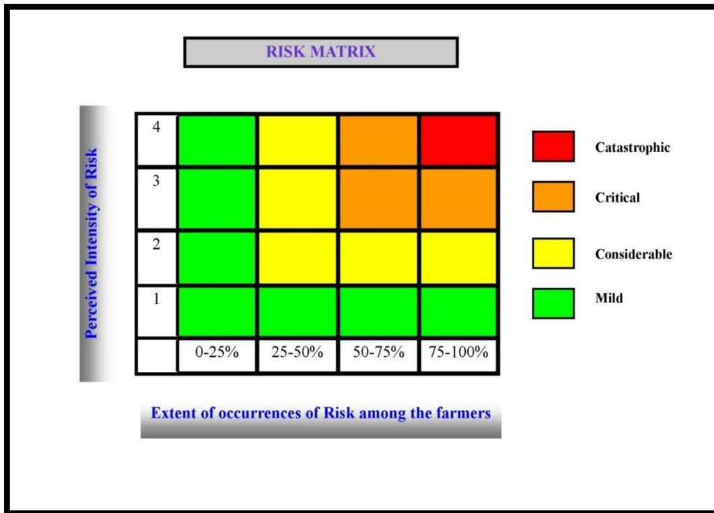
Fig. 1. Risk Matrix [7]
