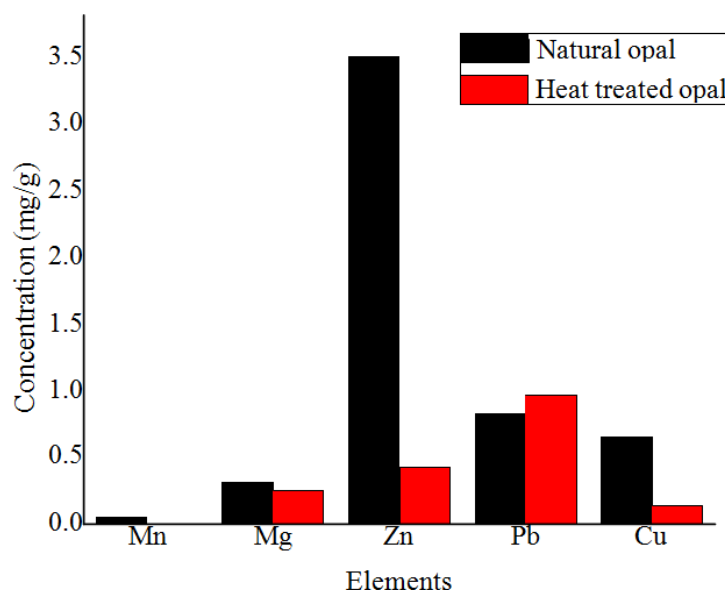
Fig. 3. The elemental composition of natural and heat treated opal
