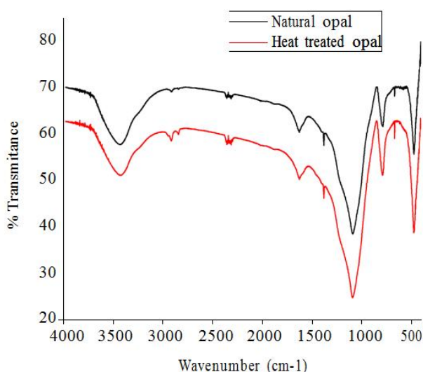
Fig. 4. FT-IR spectra of natural and heat treated opals
