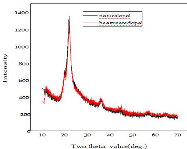
Fig. 5. The XRD pattern of natural and synthetic opals
