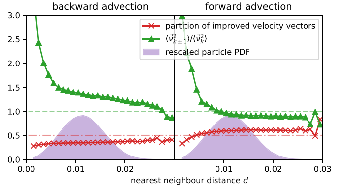
Figure 14. Velocity MSE ratios (green triangles) following VP paths after backward and forward advection in the reconstructed fields of FIT with #P = 1600 and averaged over all time steps. The partition of improved velocity vectors (red crosses) within the bulk of advected VPs. Values are binned for nearest neighbor distance to a real particle. The underlying nearest neighbor distribution is shown in violet.
