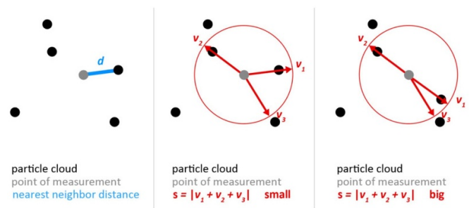
Figure 3. Sketch of the two criteria for error quantification. Left: The distance d from a measurement point (grey) to the nearest neighbor in the initial particle cloud (black). Right: The more uniform/spherical the arrangement of three nearest neighbors, the smaller s becomes.
