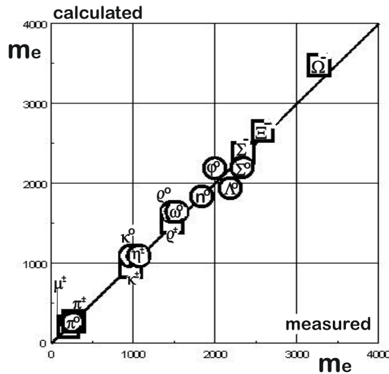
Fig. 1. Comparison of calculated values of particle masses with measurement data. Circles indicate the values of masses of neutral particles, and squares indicate masses of charged particles.
