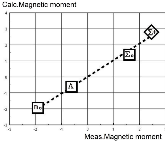
Fig. 2. Comparison of calculated values of particle magnetic moments with measurement data.
