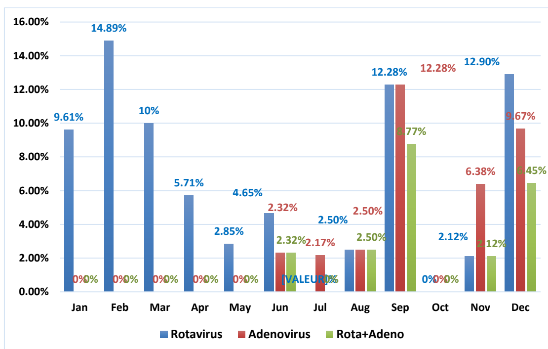
Fig. 1. Distribution of rotavirus and adenovirus positivity by month
