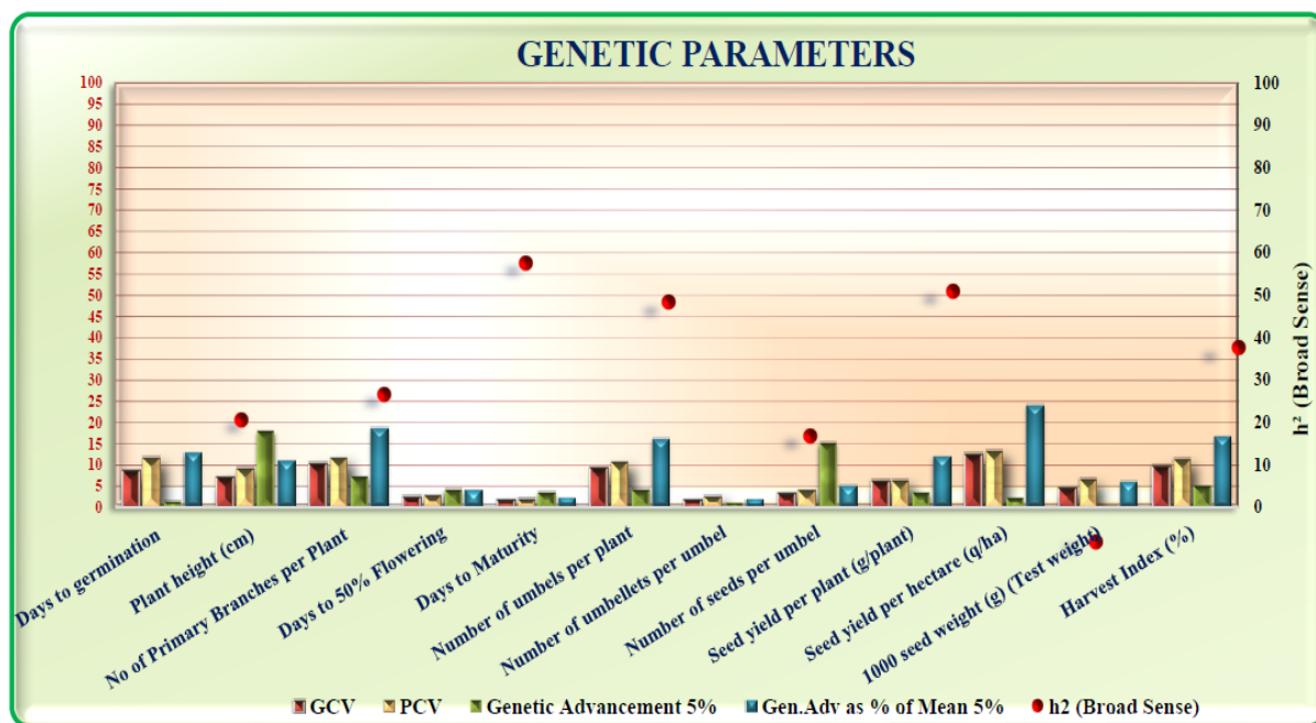
Fig. 1. Histogram representing the relationship among the GCV, PCV, Heritability, Genetic Advance and Genetic Advance as percent of mean in Fennel
