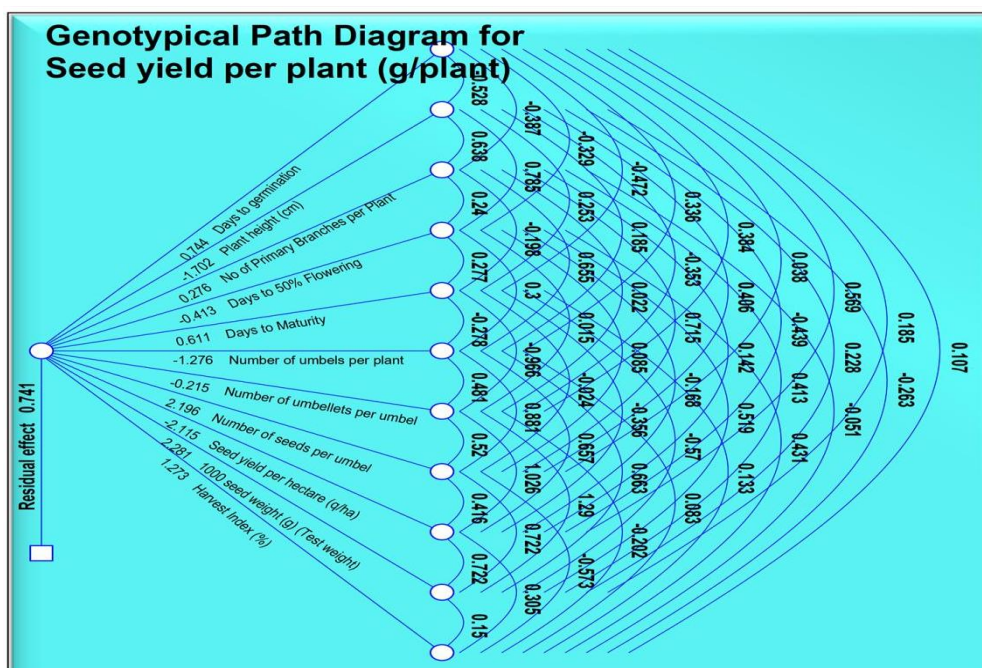
Fig. 3. Genotypic path diagram for seed yield per plant (g)
