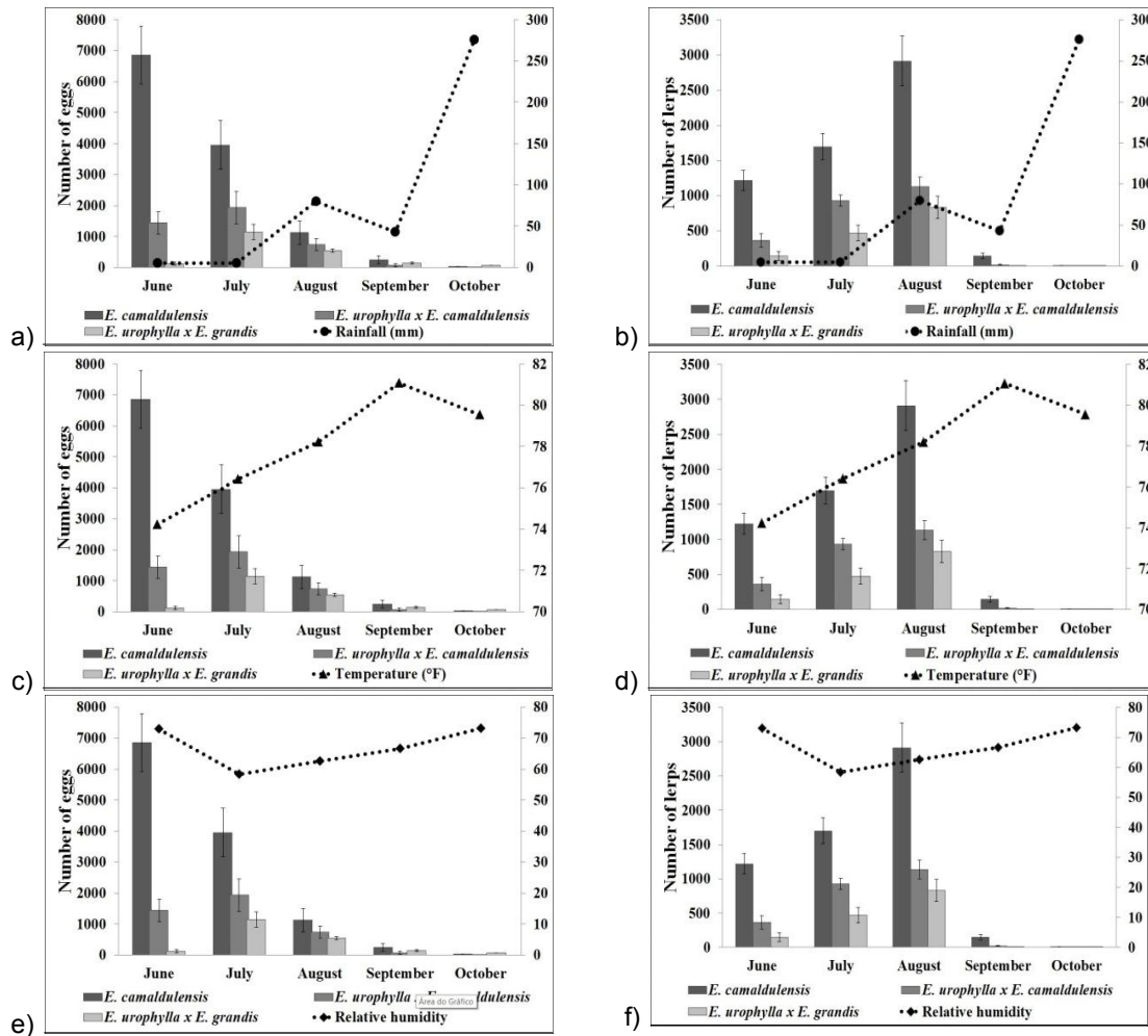
Fig. 1. Population fluctuation of eggs (a, c, e) and lerps (b, d, f) of Glycaspis brimblecombei (Moore), in Eucalyptus with respective environmental factors in Juscimeira, MT (2016)
